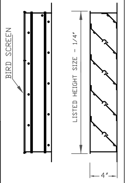
FLANGE FRAME HEAD AND SILL
