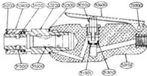
Straight Grip Type – Model 120001
