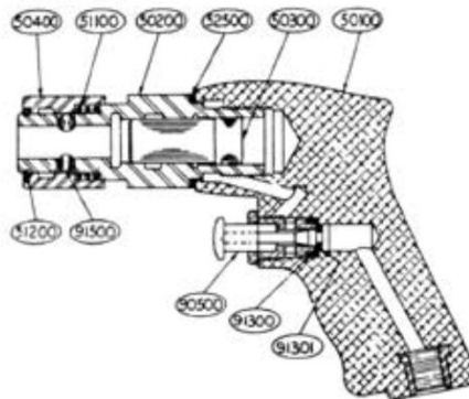
Pistol Grip Type – Model 120000
