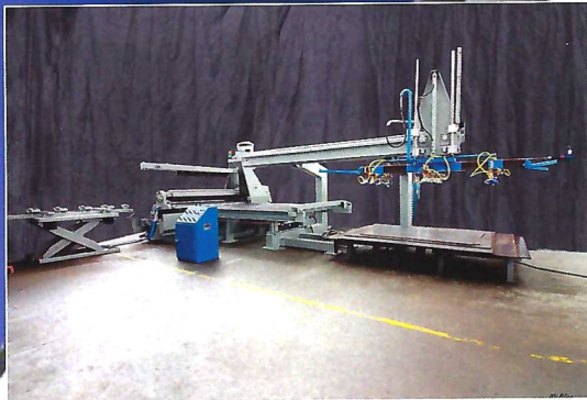
403-13-8 rolling cell to form propane tanks
