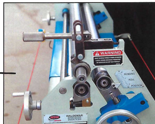
Quick release latch for swing-out top roll. Pointer and rule to show position of bending roll. Wedge and screw arrangement for accurate positioning of pinch roll.
