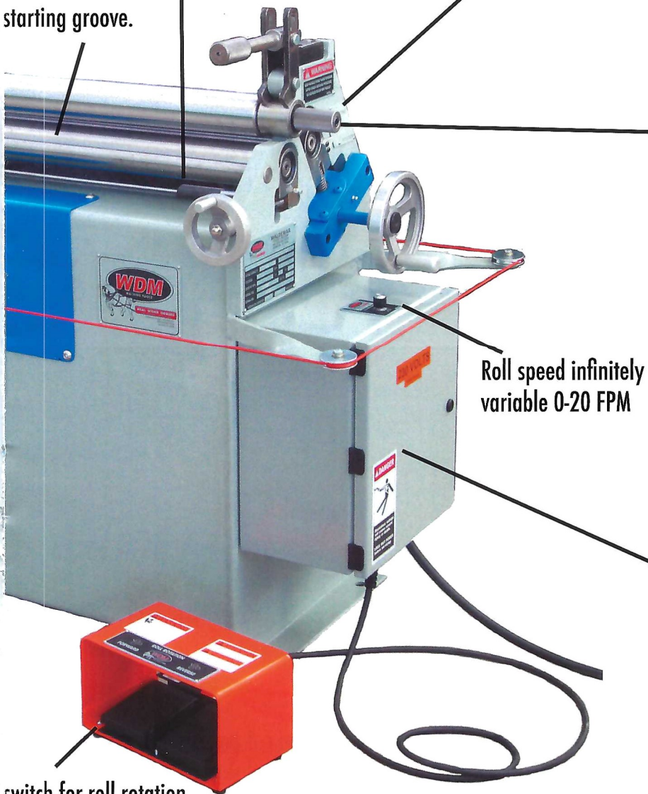
switch for roll rotation. reverse.
