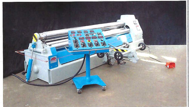
403-7-10 with rolling console and side supports
