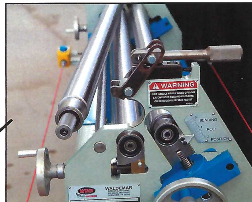
Top roll in the swing-out position to remove completed cylinder.
