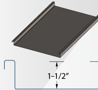
Mechanical Lock
