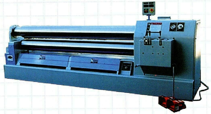
K-10-8 (13/32" x 8') This machine is equipped with optional 421 DRO to replace the dial pointer roll position.
