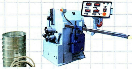
Model AR-24 (2 x 2 angle capacity) four-roll angle roll rolling machine hole rims automatically.
